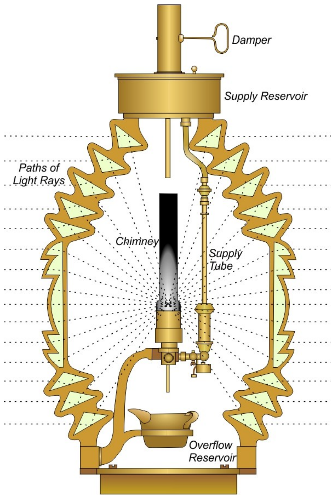
Paths of Light Rays Through a Fresnel Lens (Based on the drawing by Frank Perry)
